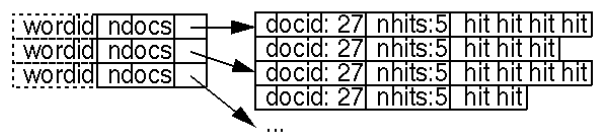
Figure 3. Forward and Reverse Indexes and the Lexicon
