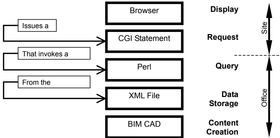
Figure 2 .The process of retrieving the information from the XML file through the web
