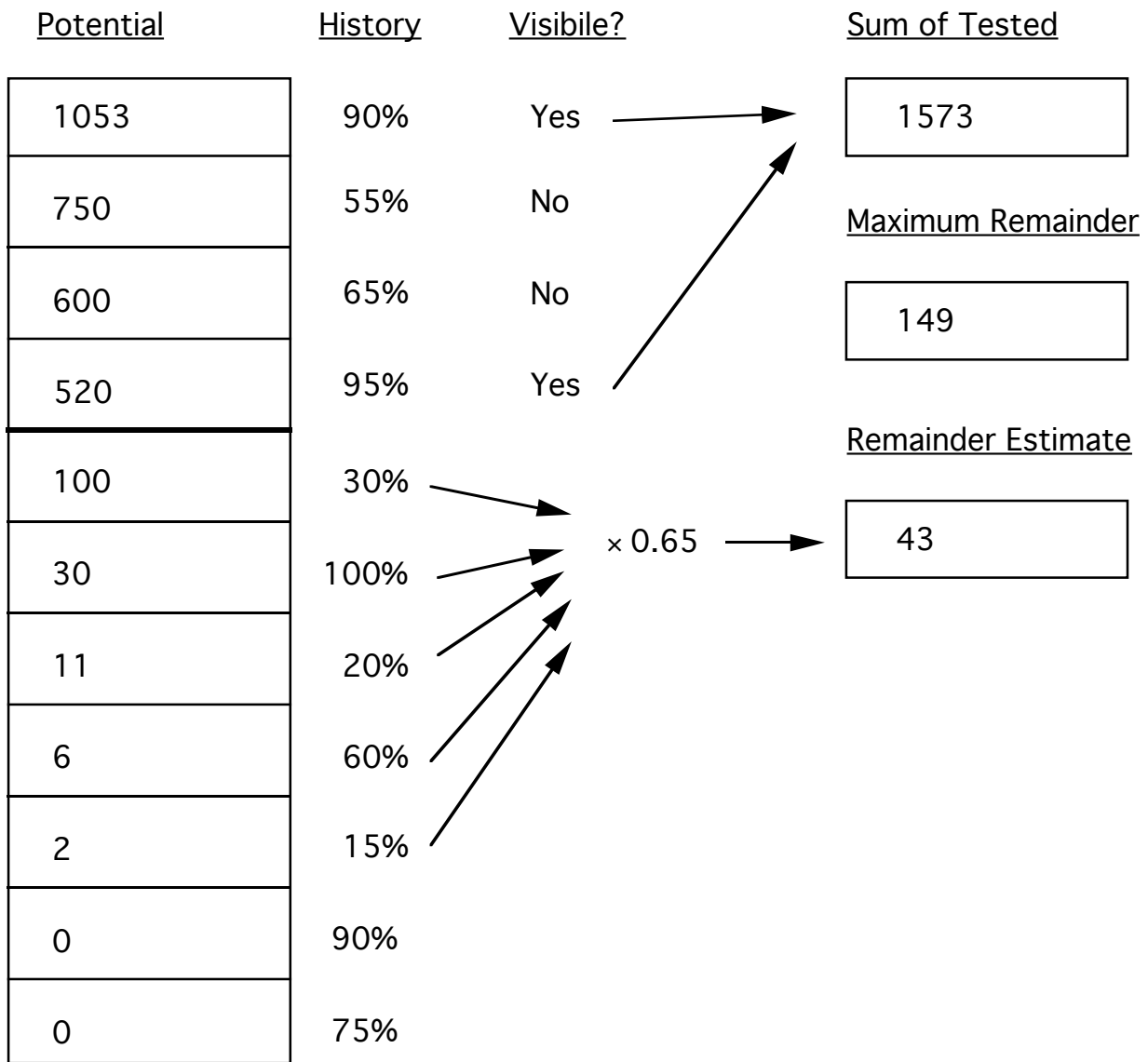
Figure 4 : Adaptive shadow testing algorithm, explained in Section 3.4.
