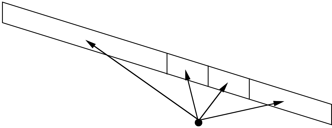
Figure 6a : Linear light source is adaptively split to minimize falloff and visibility errors.
