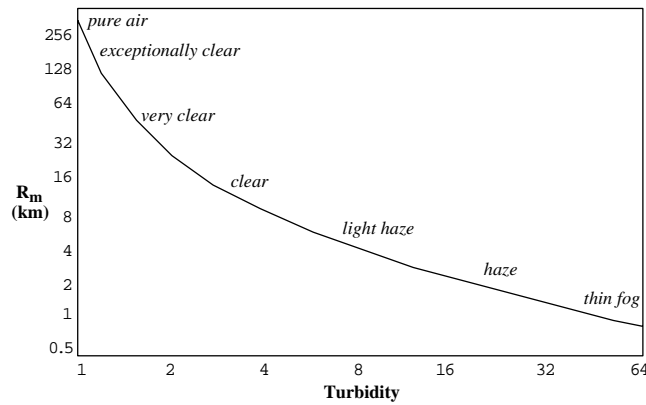
Figure 3: Meteorological range R_m for various turbidity values. Values computed from source data in McCartney [19]
