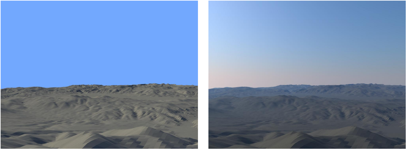
Figure 1: Left: A rendered image of an outdoor scene with a constant colored sky and no aerial perspective. Right: The same image with a physically-based sky model and physically-based aerial perspective.
