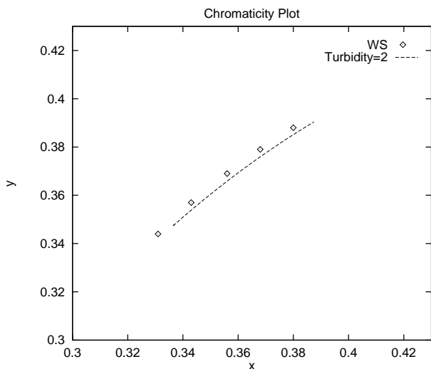
Figure 7: Plots of chromaticity values of sunlight for turbidity 2, compared with data from Wyzsecki and Stiles. Sun angles considered are from 0 to 78.5 degrees.
