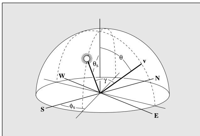
Figure 4: The coordinates for specifying the sun position and the direction \mathbf{v} on the sky dome.
