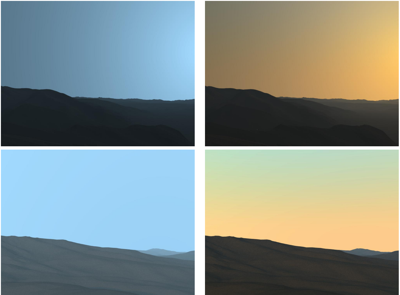
Figure 11: Left: the CIE clear sky model using constant chromaticity coordinates and Ward's aerial perspective approximation for west and east viewing directions and the same viewpoint. Right: the new model. Note the change in hue for different parts of the sky for the new model.
