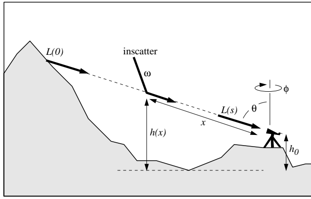
Figure 8: The variables used to compute aerial perspective.
