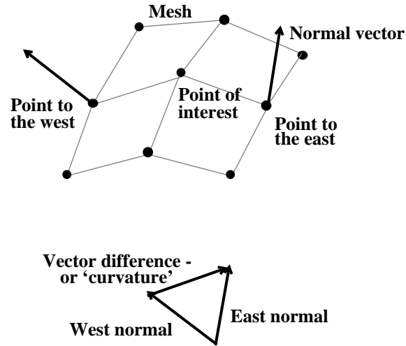
Figure 8. Vector Difference to represent Curvature
