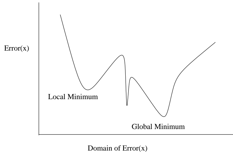
Figure 10. Local Minima in an Error Function
