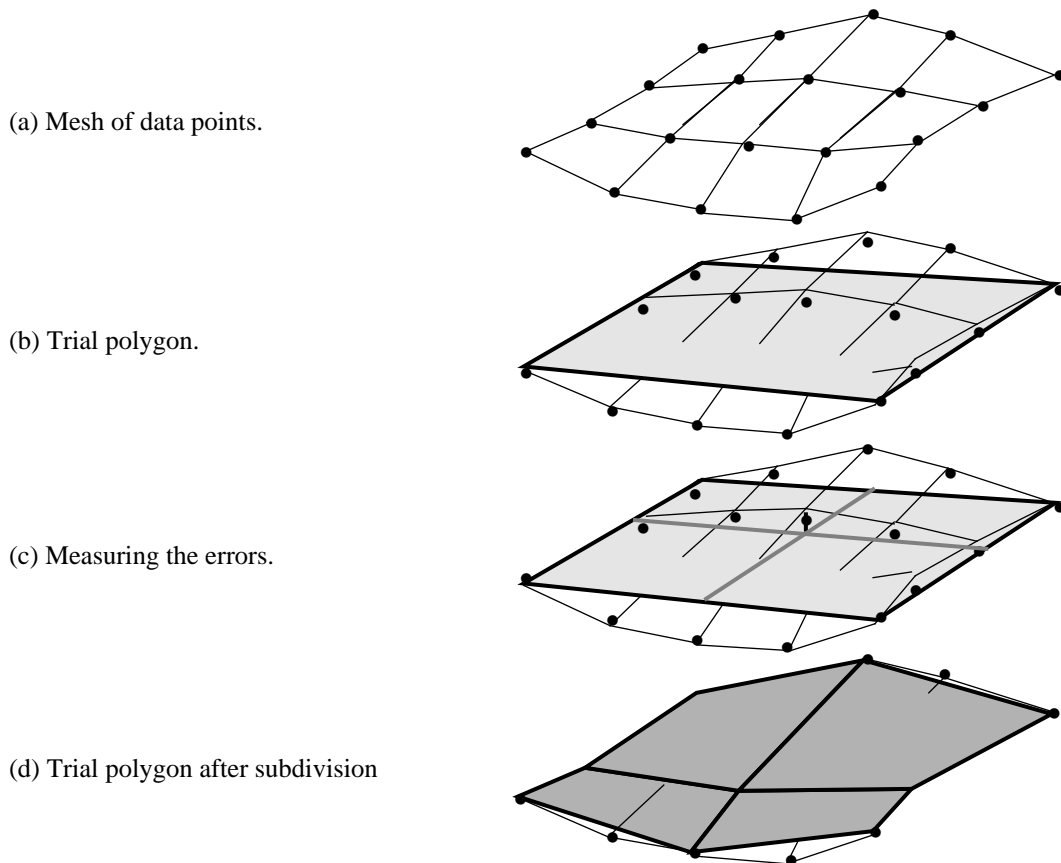
Figure 3. Surface-fitting Polygons with Adaptive Subdivision
