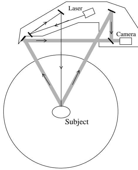
Figure 1. Schematic View of Cyberware Digitizer
