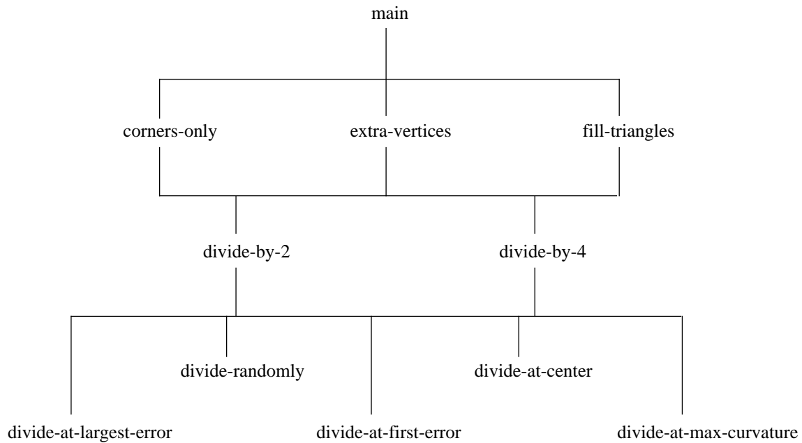
Figure 5. Adaptive Subdivision Variation Hierarchy
