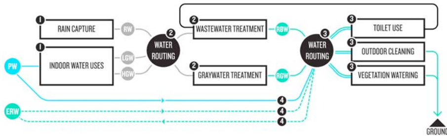
Figure 1. Proposed Simulation Process (ERW = External Recycled Water; PW = Potable Water; LGW = Light Graywater; HGW = Heavy Graywater; RGW = Recycled Graywater; RBW = Recycled Blackwater)
