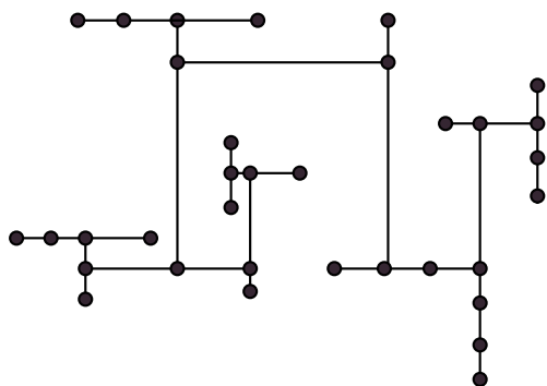
Fig 3. H-tree layout
