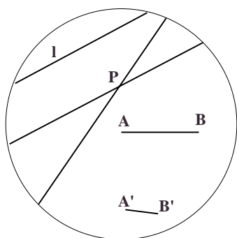
Fig. 12. The Klein for the hyperbolic plane. The line segments AB and A'B' have an equal length in the hyperbolic sense.
