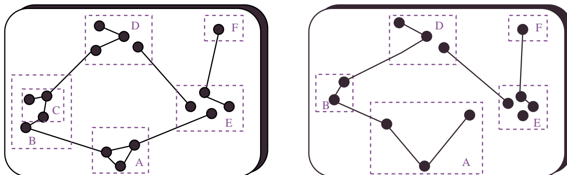
Fig. 19. Multifocal fisheye/zoom in a hierarchically clustered graph. The dotted rectangles denote the (logical) clusters. Note the disappearance of cluster C on the right hand side. (Adapted from Schaffer et al. [112].)
