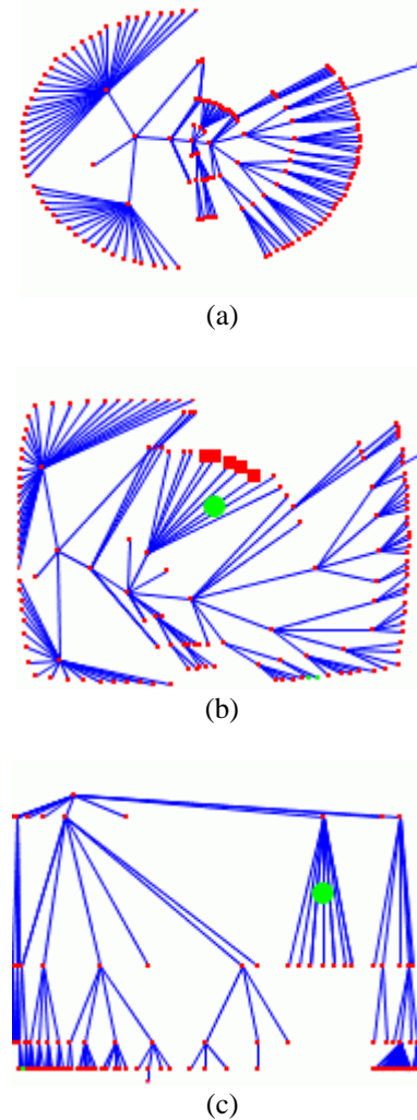
Fig 16. Fisheye distortion. Figure (a) represents the graph without the fisheye. Figure (b) uses polar fisheye, whereas Figure (c) uses cartesian fisheye with a different layout of the same graph. The green dots on Figures (b) and (c) denote the focal points of the fisheye distortion. Note the extra edge-crossing on Figure (b).
