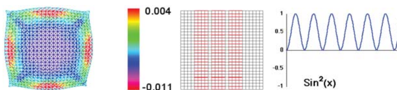
Figure 4: Left: Gaussian curvature representation indicating areas of positive and negative curvature in the mesh. Right: Increasing the length of red regions driven by a \text{Sin}^2(x) curve introduces intrinsic deformation to the mesh.
