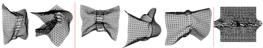
Figure 5: Digital simulation of resin impregnation which is applied perpendicular (left) and parallel (right) to stretch
