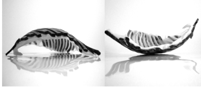
Figure 2: Resin impregnated latex-membrane physical experiment (left and right - frontal and dorsal elevation views) demonstrating curvature induced by pre-stretching.
