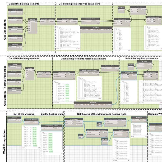
Figure 3. Extracting directly accessible and indirectly accessible parameters from a Revit model in Dynamo.
