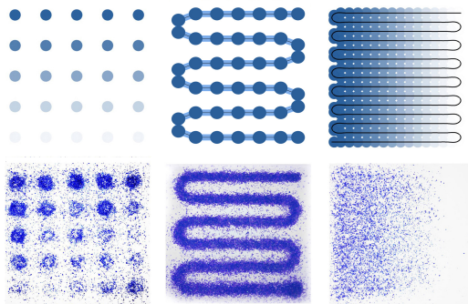
Figure 5. Dispensing a) discrete dots b) along a continuous curve c) along a continuous curve with varying speed and decreased distance.
