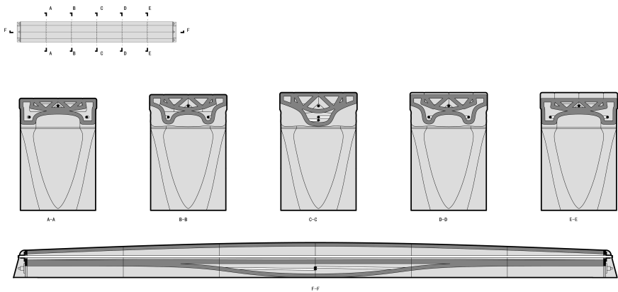
Figure 6. section drawings.
