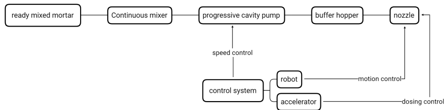
Figure 3. extrusion process.
