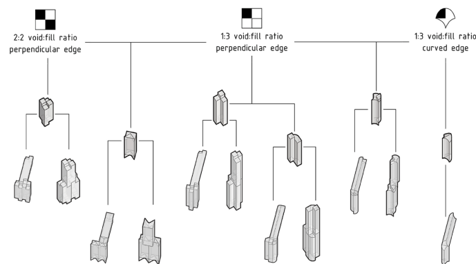
Figure 4. Exploration of tessellating and interlocking geometry, through evaluation of vertical to horizontal joinery.
