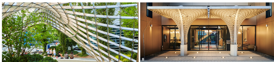
Figure 1. Asymptotic lamella gridshells. A: The Inside/Out Pavilion at the Technical University in Munich. B: The Intergroup Hotel Canopy in Ingolstadt.
