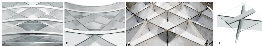
Figure 9. Developable strip facade along the principal curvature directions.
