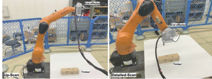
Figure 5. The screenshot of each scanning moment and robot attitude ;(case-1) Up-scan is the rough scan of the procedure following 0, 1, 2,( see table 3) ;(case-2) Detailed-Scan is the procedure following 0,1,2,(3,4), 5 (see table 3)
