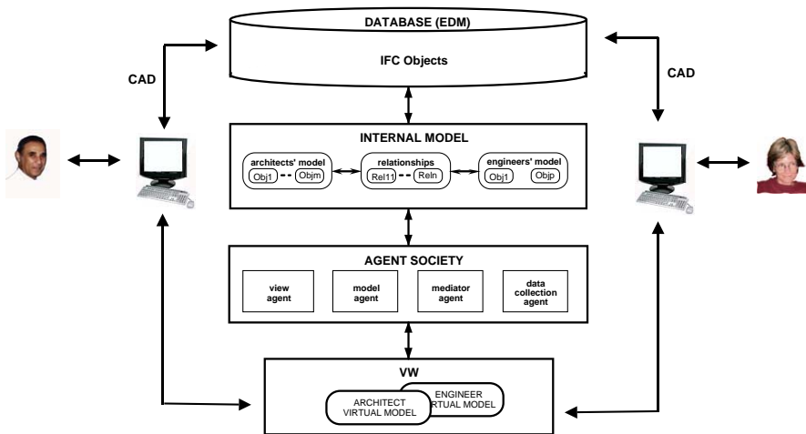
Figure 3 System architecture
