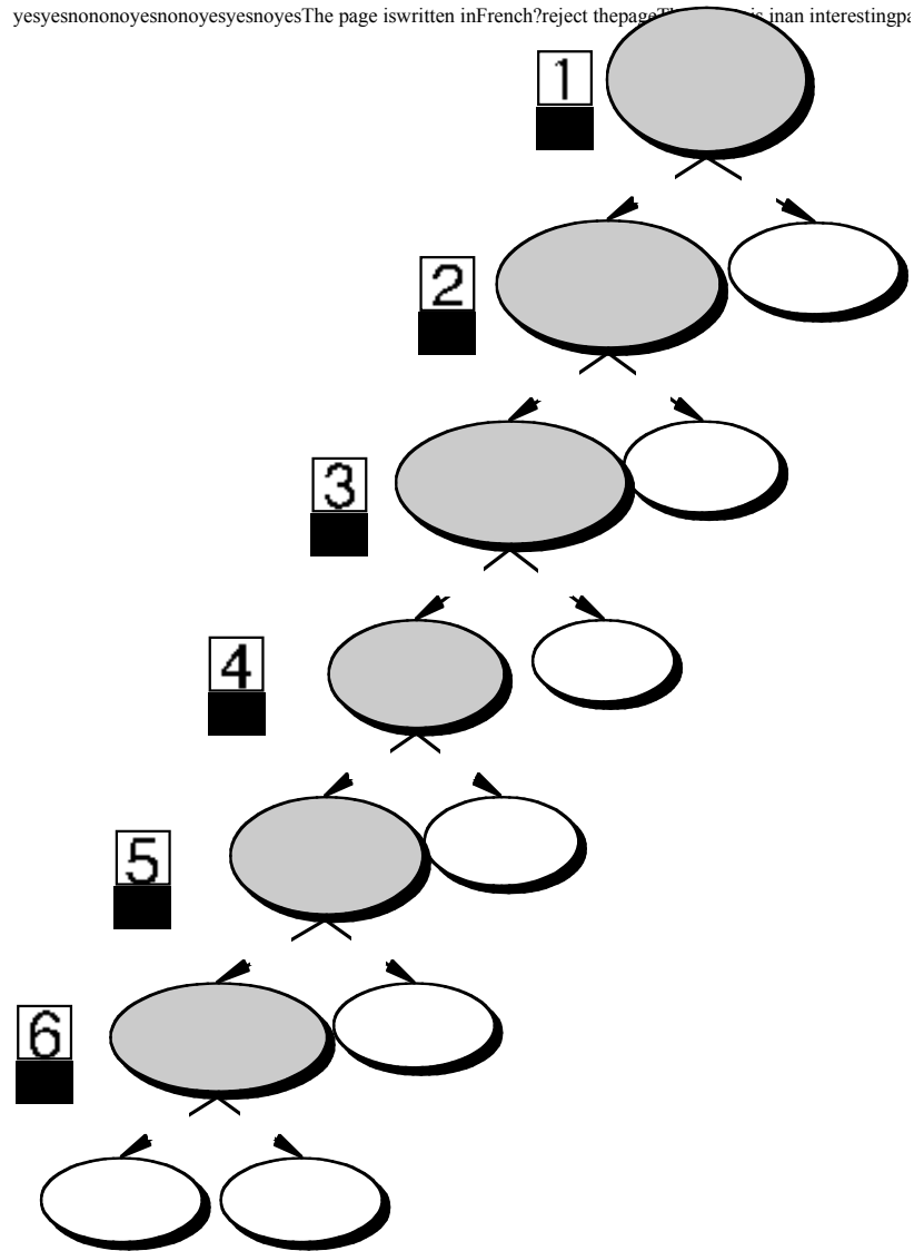
Figure 1: Decision tree
