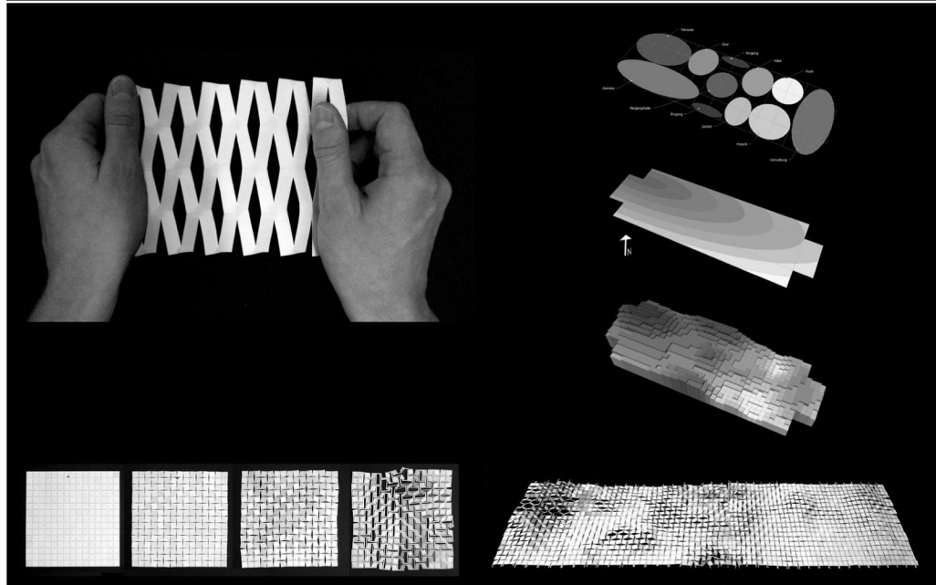
Figure 12 “The principle of expanded metal is used to create a parametric sunshade system. The size of the openings are controlled by the position and length of the incisions”, student design project, winter 06/07, Fabio Fichter, Saskia Mayer, Technical University of Darmstadt
