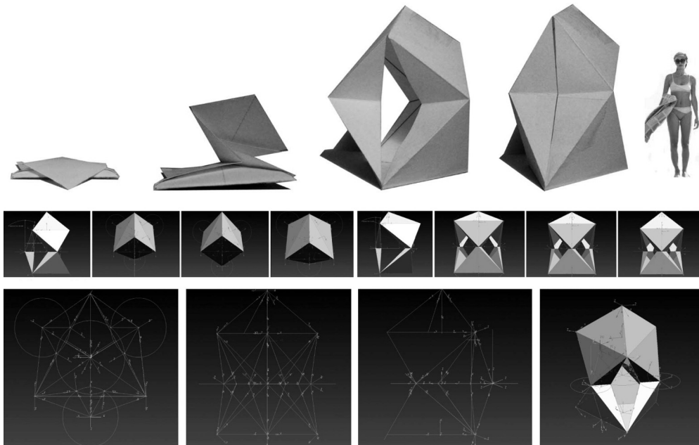
Figure 10 "Folding beachcabin and parametric model in Unigraphics", student design project, winter 06/07, Edda Gaudier, Stephan Mehlhorn, Susann Zimmermann, Technical University of Darmstadt
