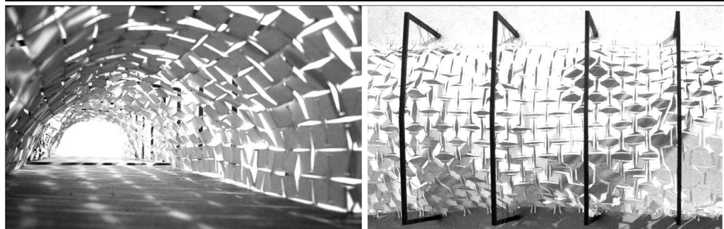
Figure 13 “Sunshade structure with parametric openings ac- cording to site orientation and internal usage”, student design project, winter 06/07, Fabio Fichter, Saskia Mayer, Technical University of Darmstadt
