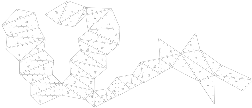
Figure 15 The subdivided surface was unfolded. Facets were then reconnected to create a 2D model
