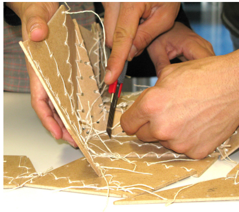
Figure 16 (left) Assembling panels by string
