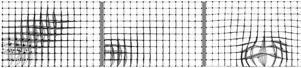
Figure 1 FiberGrid; Screenshots.
