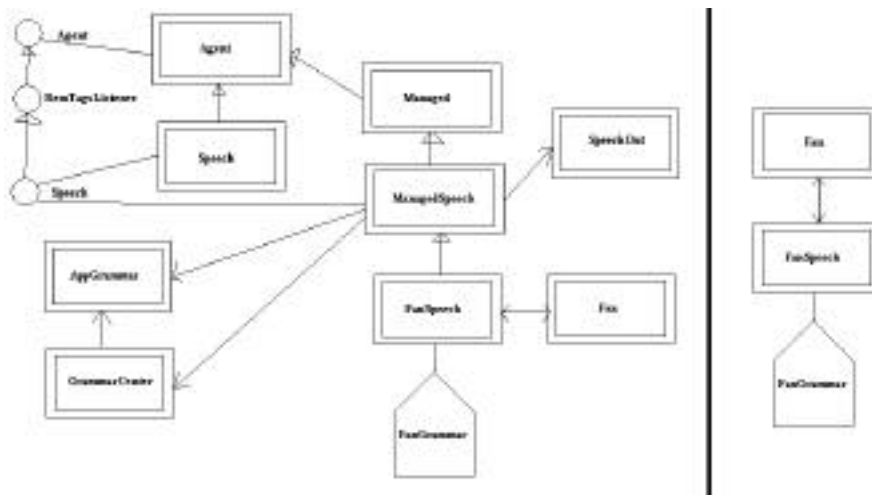
Figure 5. The left shows the speech grammar along with connected classes. The right shows the simpler version with the grammar symbol implying the relationships and agents on the left.
