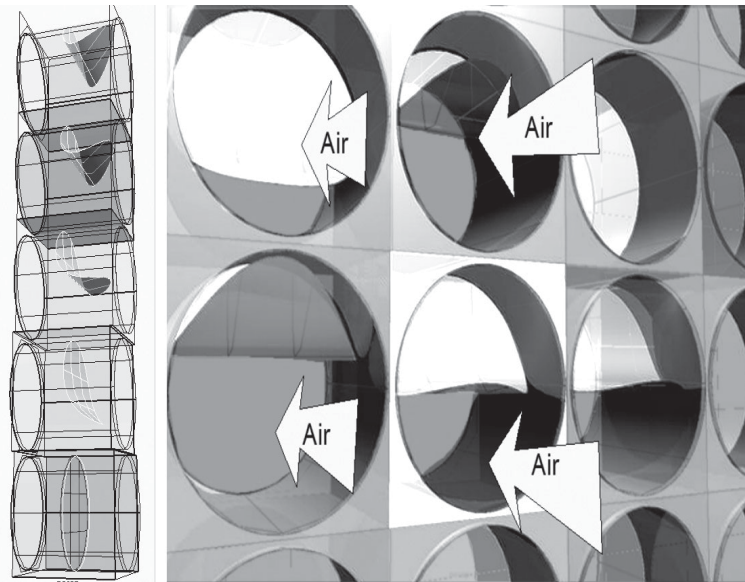
Figure 3. Smart shape memory alloy membranes at micropores for air circulation through wall
