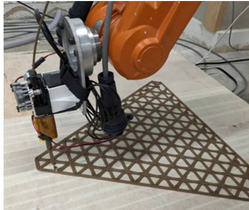
Figure 7 Photos of the Printing Process Using 20:80 Composite
